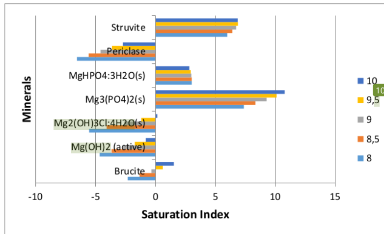
1 Figure 1. Modeling results of minerals from MINTEQ calculation
