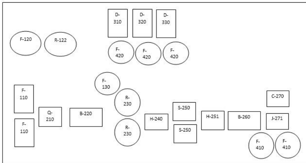
Gambar I.6.2. Lay Out Peralatan Pabrik
