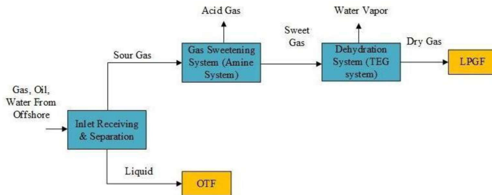
Gambar II. 4 Diagram Blok Gas Processing Facilities (GPF)
