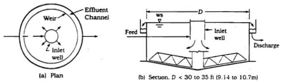
Gambar 2. 8 Bak Pengendap Circular
