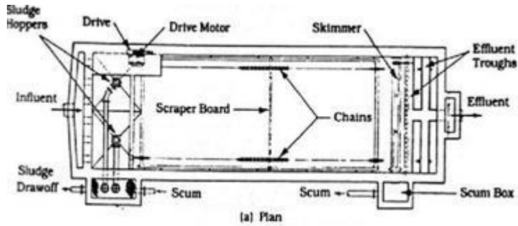
Gambar 2. 6 Denah Bak Pengendap Rectangular
