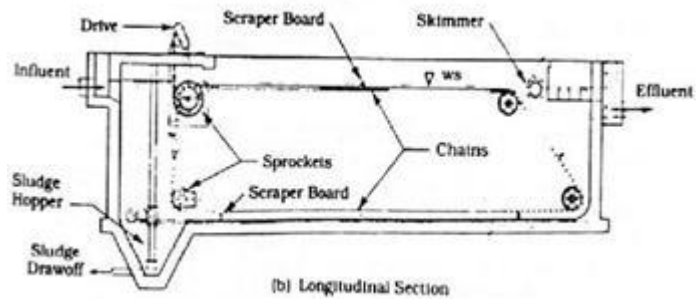
Gambar 2. 7 Potongan Samping Bak Pengendap Rectangular
