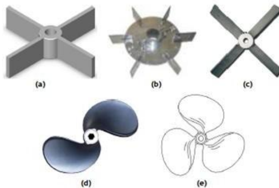
Gambar 2. 3 Tipe Turbine Impeller
