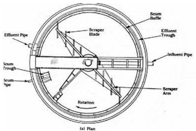
Gambar 2. 12 Potongan Clarifier
