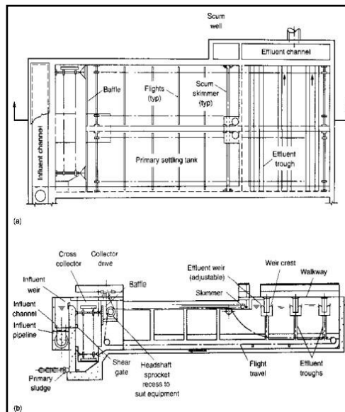
Gambar 2. 5 Bak Sedimentasi (a) denah (b) potongan
