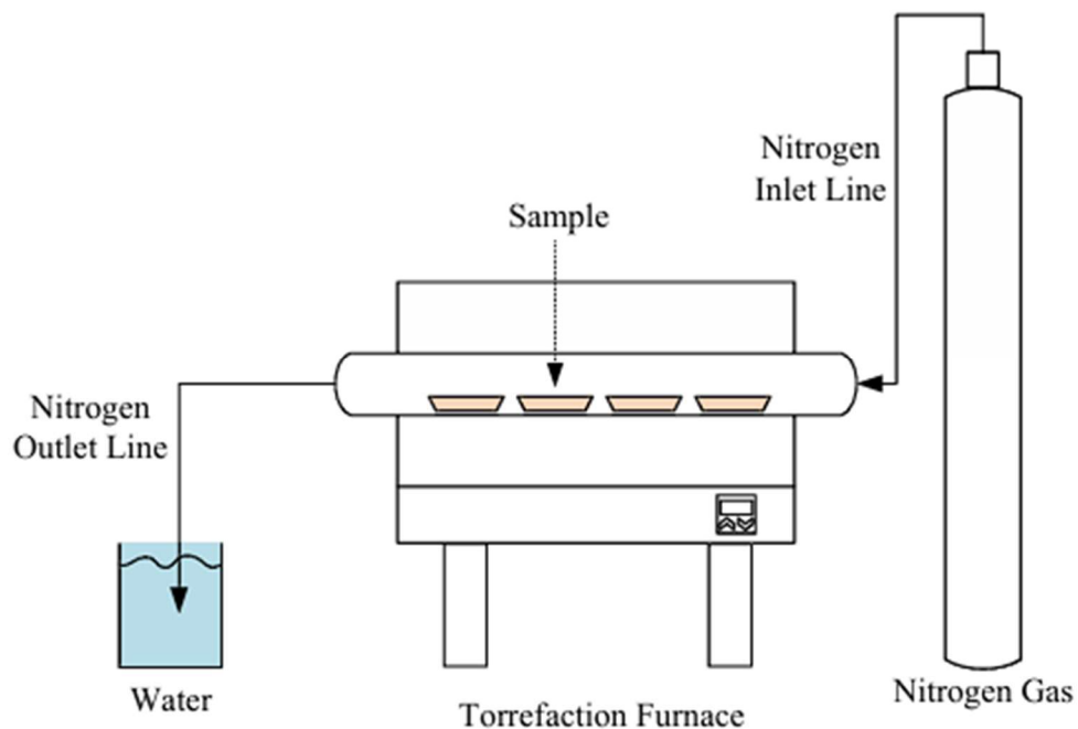
Gambar III. 1 Rangkaian Alat Penelitian
