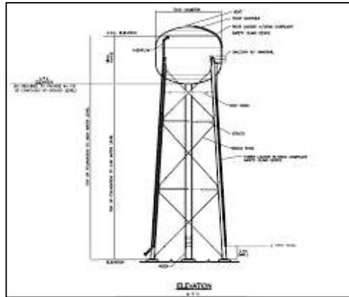
Gambar 2. 14 Reservoir Menara
