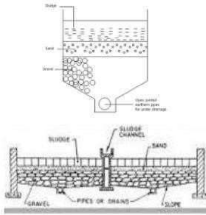
Gambar 2. 18 Sludge Drying Bed
