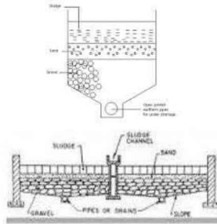
Gambar 2 18 Sludge Drying Bed
