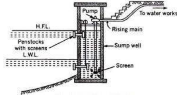
Gambar 2. 1 River Intake
