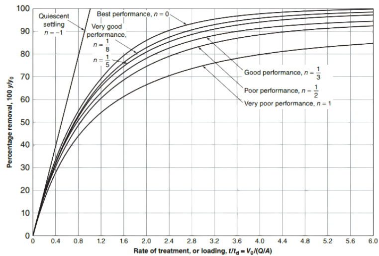
Gambar 2 10 Performance curves for settling basins of varying effectiveness
