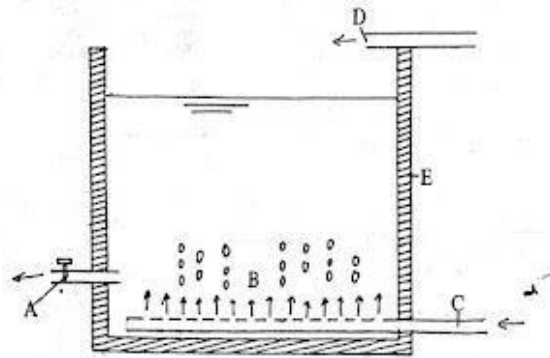
Gambar 2. 2 Bubble Aerator
