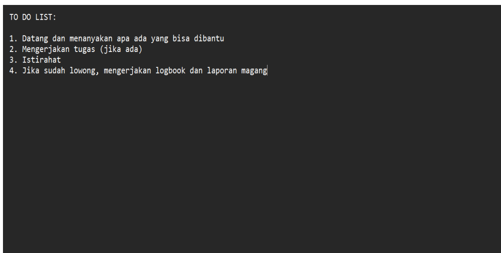
Gambar 21 (Membuat To-do-list )
