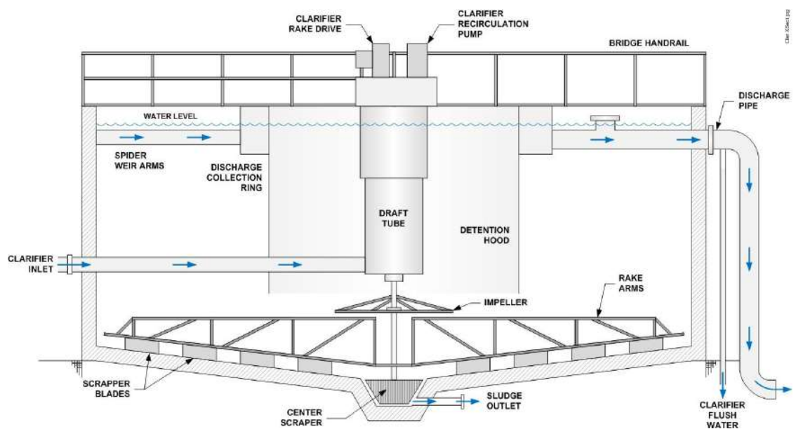
Gambar 2. 6 Clarifier
