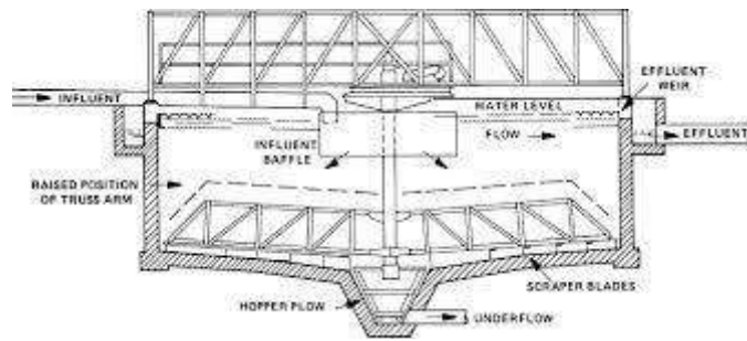
Gambar 2. 8 Sludge Thickener
