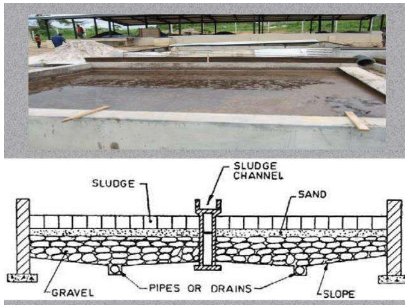
Gambar 2. 7 Sludge Drying Bed
