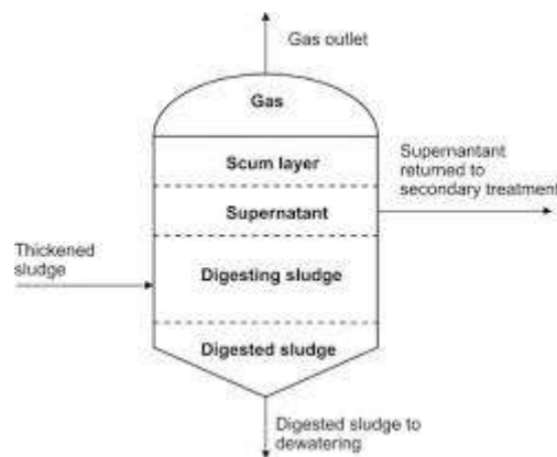
Gambar 2. 9 Sludge Digester
