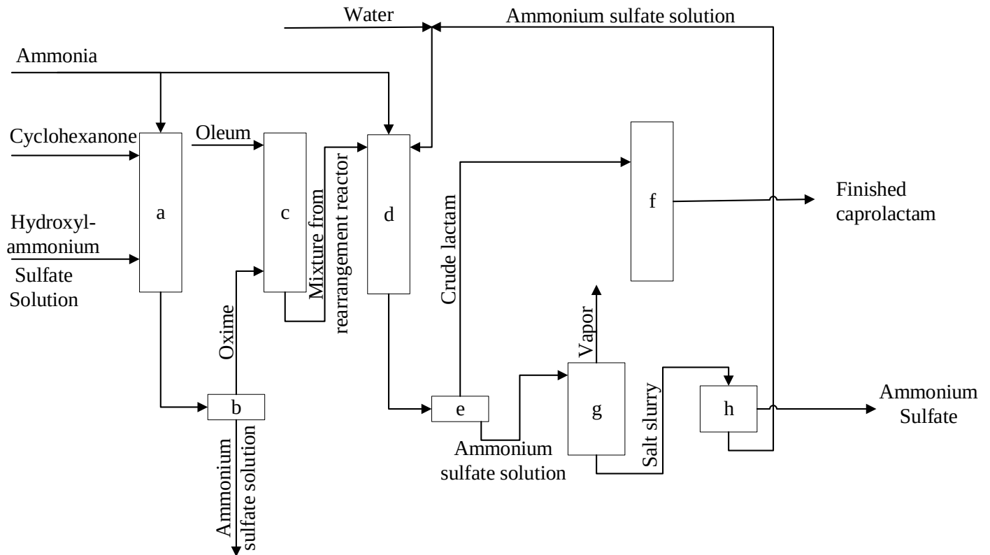
Gambar II.1 Blok Diagram Proses Rearrangement Beckmann
