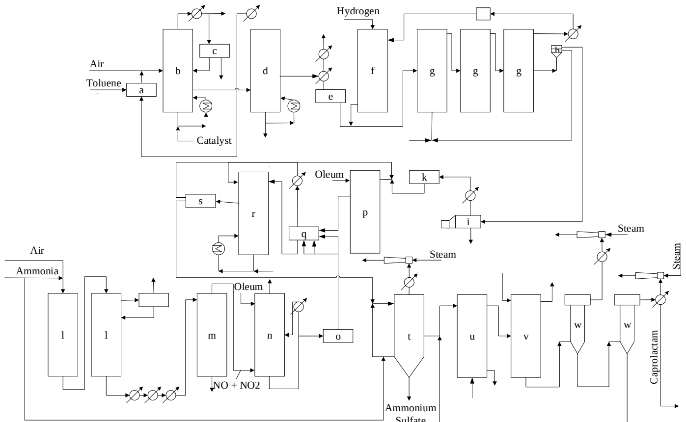
Gambar II.2 Blok Diagram SNIA Viscosa Process
