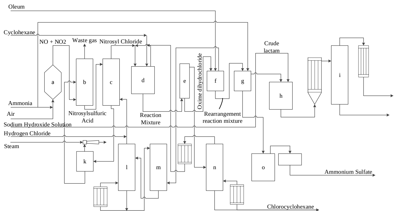
Gambar II.3 Blok Diagram Proses Toray
