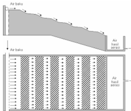
Gambar 2. 8 Submerged Cascade Aerator
