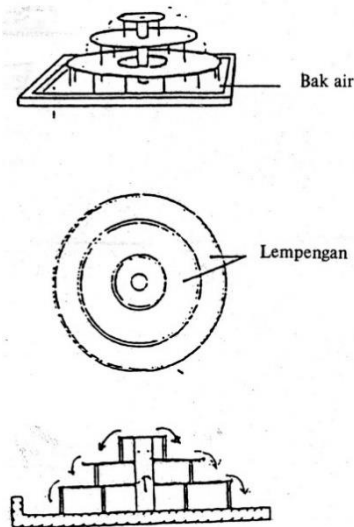
Gambar 2. 9 Multiple Platform Aerator
