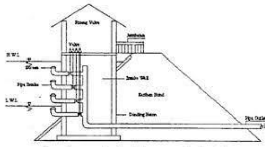
Gambar 2. 5 Reservoir Intake
