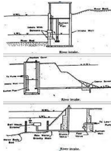
Gambar 2. 3 River Intake
