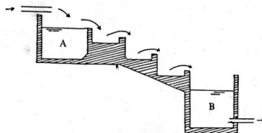
Gambar 2. 7 Cascade Aerator
