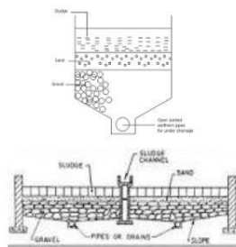
Gambar 2. 25 Sludge Drying Bed
