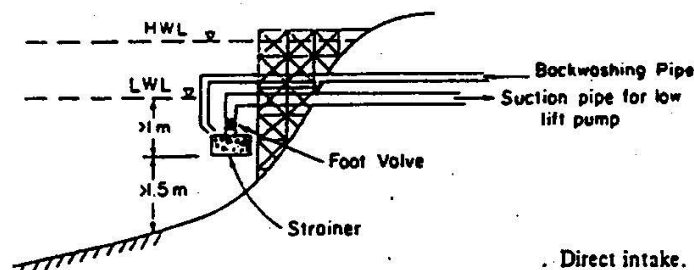
Gambar 2. 2 Direct Intake
