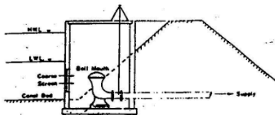
Gambar 2. 4 Canal Intake
