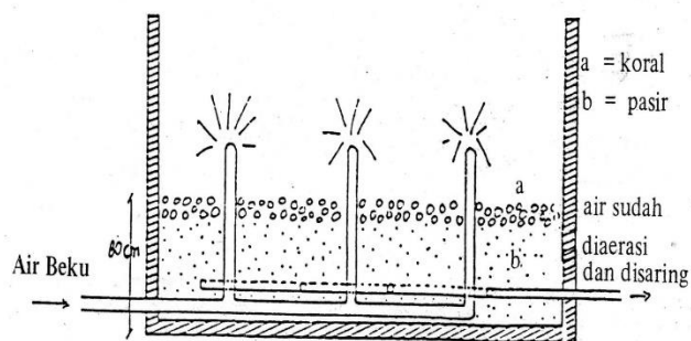
Gambar 2. 10 Spray Aerator
