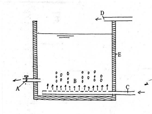
Gambar 2. 11 Bubble Aerator
