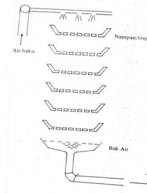
Gambar 2. 6 Waterfall Aerator
