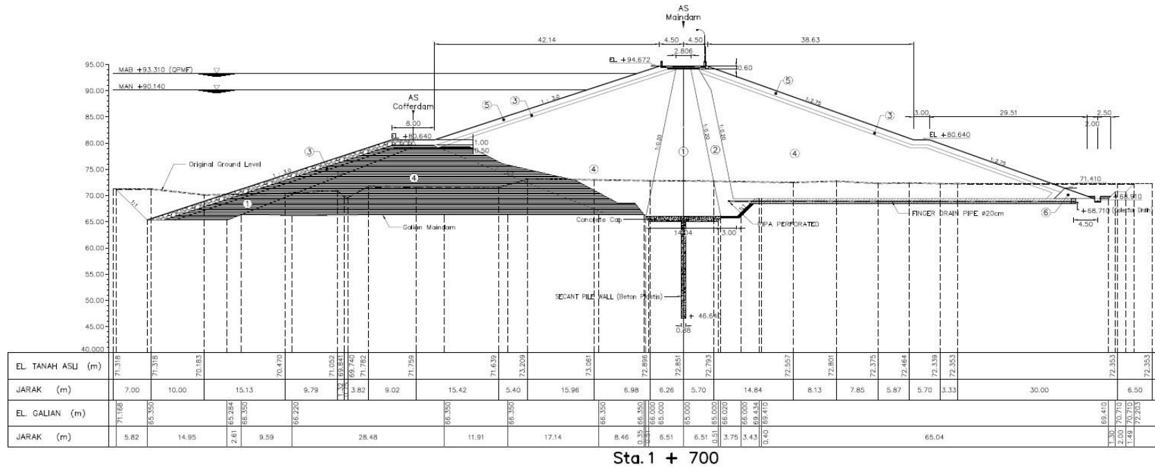
Lampiran 1 Gambar cross section main dam bendungan semantok
