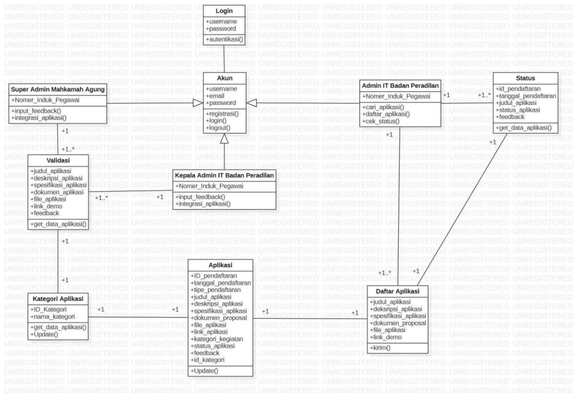
Gambar 18 Class Diagram
