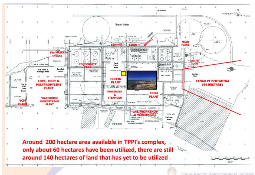
Gambar 6. Denah PT TPPI Plant Tuban
