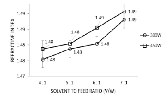
Fig. 2. Effects of Solvent to Feed Ratio and Microwave Power on Refractive Index of Essential Oil from Red Guava Leaves
