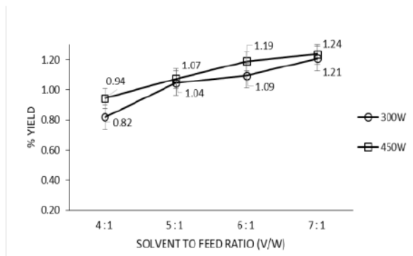
Fig. 1. Effects of Solvent to Feed Ratio and Microwave Power on Yield of Essential Oil from Red Guava Leaves
