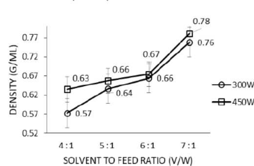
Fig. 3. Effects of Solvent to Feed Ratio and Microwave Power on Density of Essential Oil from Red Guava Leaf
