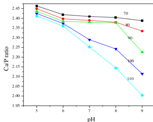
Figure 1. Effect of pH on Ca/P ratio
