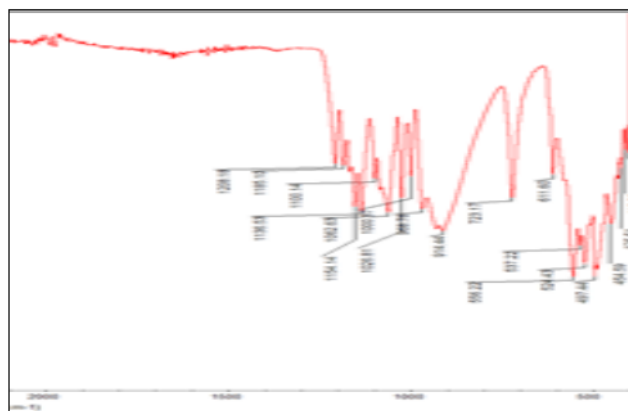
Figure 3. IR Spectra for Calcium Phosphate at 800 °C
