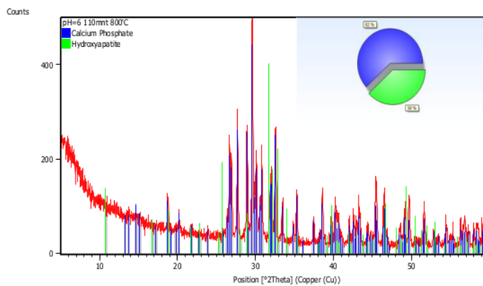
Figure 2. XRD for Calcium Phosphate at 800 °C
