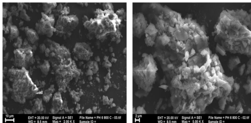
Figure 4. IR SEM image Calcium Phosphate product at 800 °C
