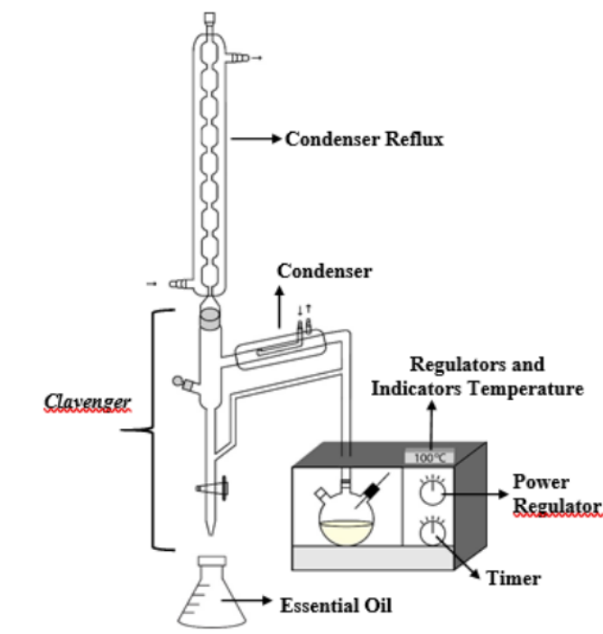
Figure 1. Schematic of the Research Tool for Extracting Essential Oils from Crystal Guava Leaves Using the Microwave Hydrodistillation Method
