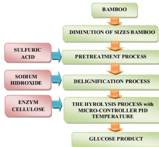
Fig. 3. Block diagram of glucose production from bamboo fitted microcontroller PID
