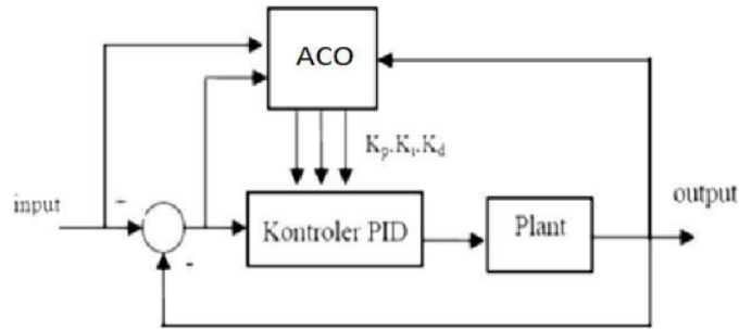
Fig. 1. Controller PID-ACO for plant
