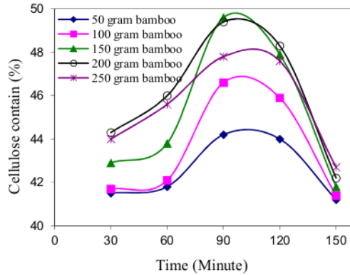
Fig. 4. Contains cellulose function hydrolysis time
