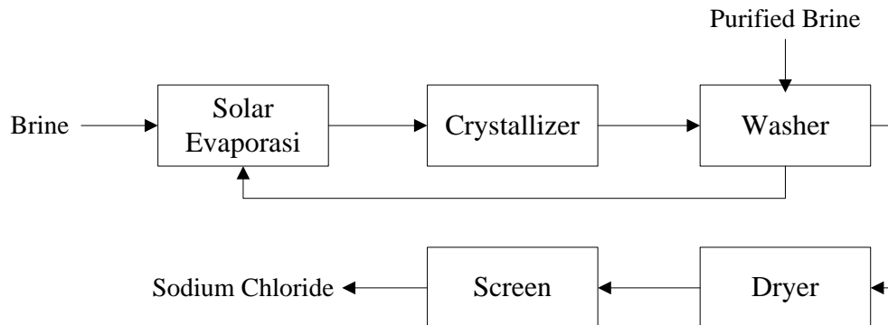
Gambar II. 1 Diagram Proses Sistem Solar Evaporation
