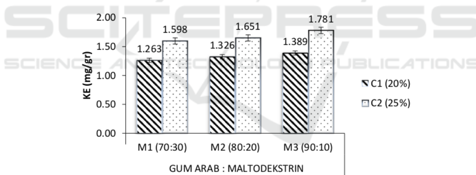
Figure 1: Histogram of KE (trapped capsaisin) values on encapsulation of chili powder.
