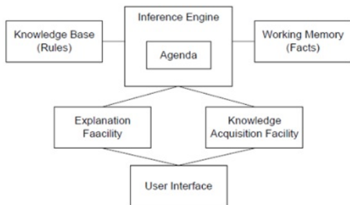
Figure 1. Expert System structure
