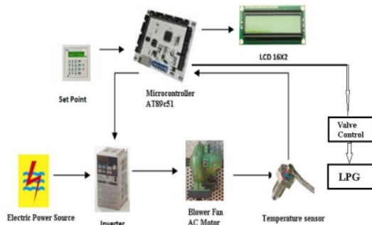
Figure 4. Diagram of the dryer working system
