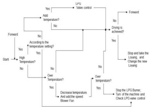
Figure 3. Decision Diagram Expert System
