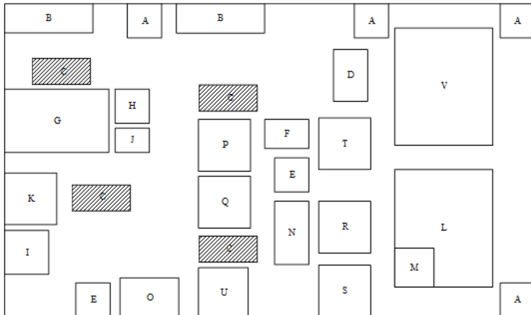
Gambar I.1 Lay Out Pabrik Silika Precipitated
