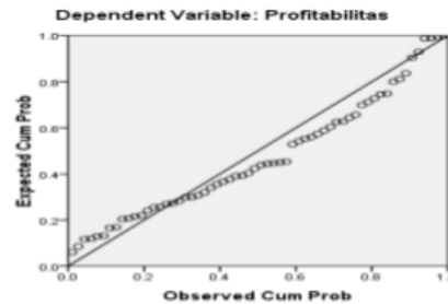
Figure 1: Graph of scatterplot Normality
