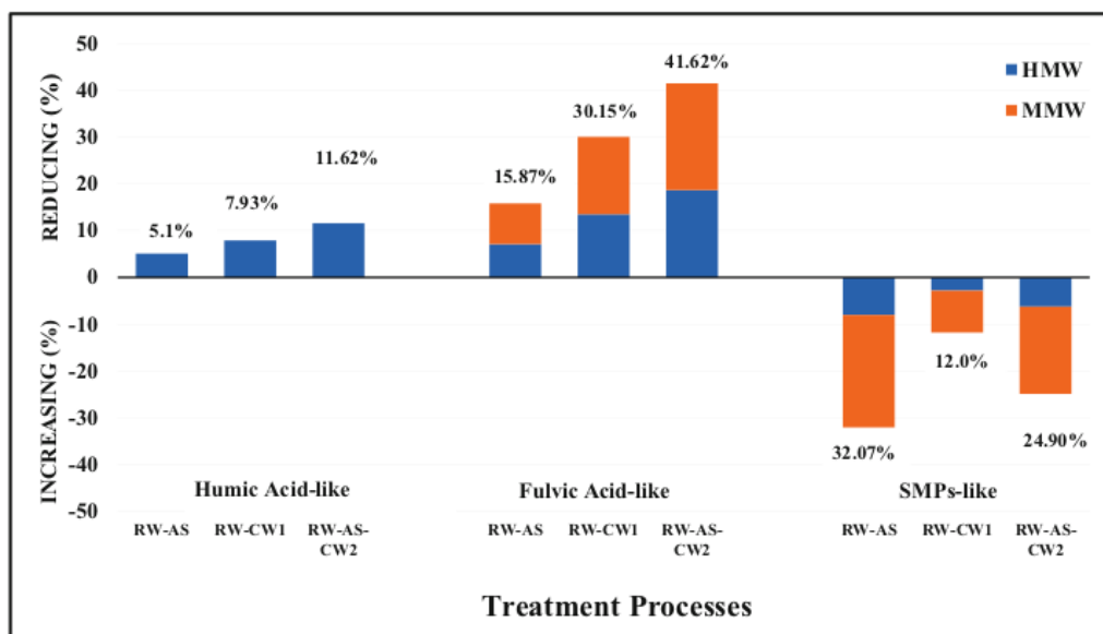
Fig. 5 Average percentage reducing and increasing in the area of each peak of HPSEC-FLD chromatogram after various treatments
