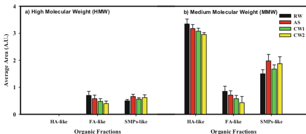
Fig. 4 Average of peak area of a HMW and b MMW of the HPSEC-FLD chromatograms in all samples by peak-fittings
