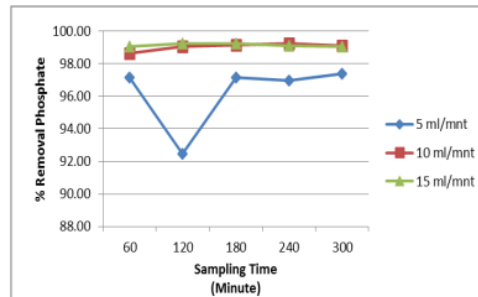
Figure 3. Relations of time sampling with percent allowance in various flow at high adsorbent 20 cm
