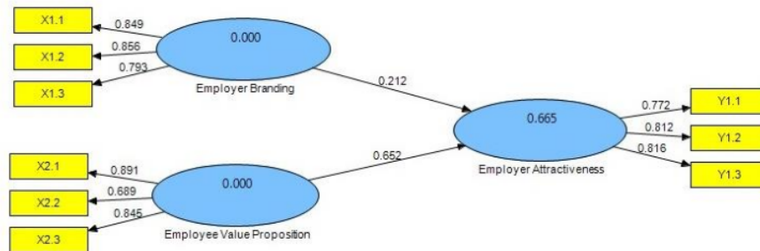
Figure 2. Conceptual with Factor Loading, Path Coefficient, and R-Square
