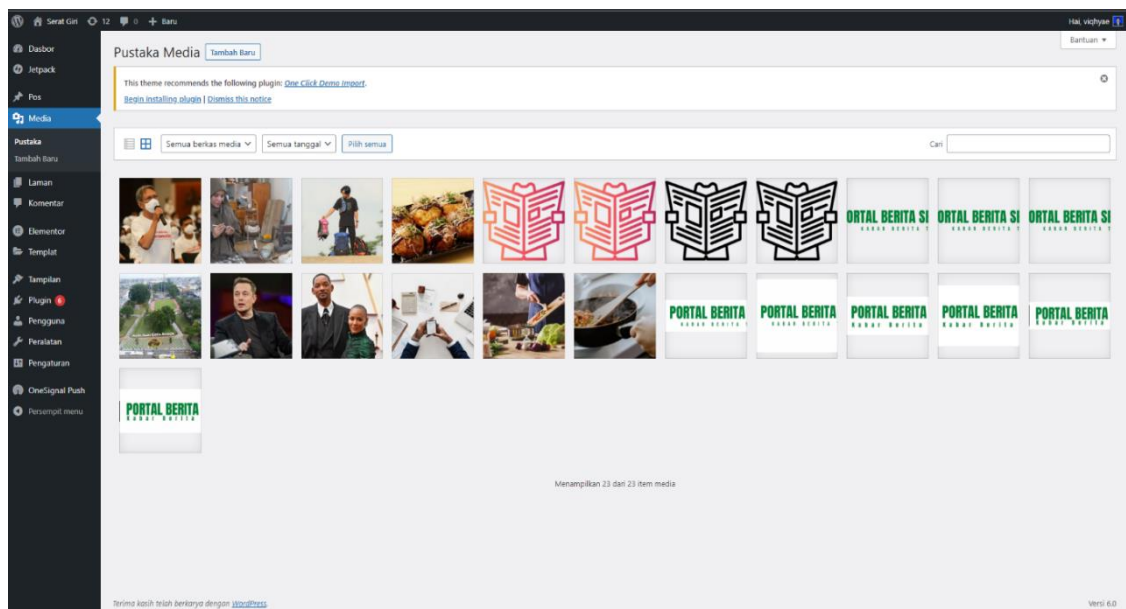
Gambar 2.5 Fitur Media
