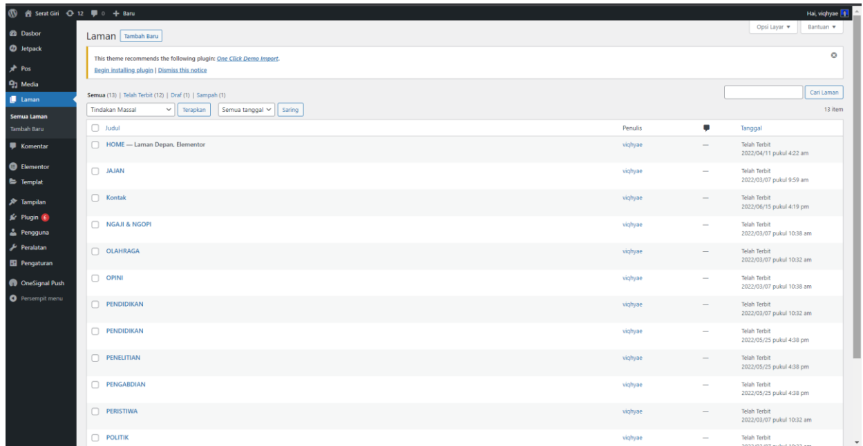
Gambar 2.6 Fitur Laman
