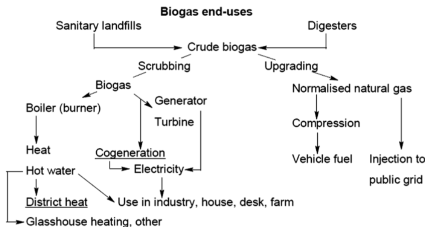
Figure 1. The overview of biogas utilization
