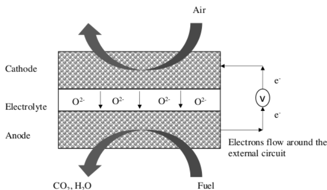
Figure 2. The schematic working principle of SOFC
