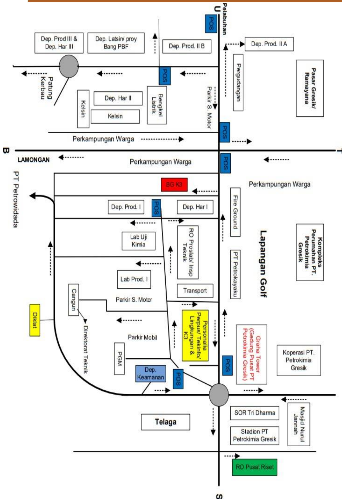
Gambar I. 3 Plant Layout PT. Petrokimia Gresik
