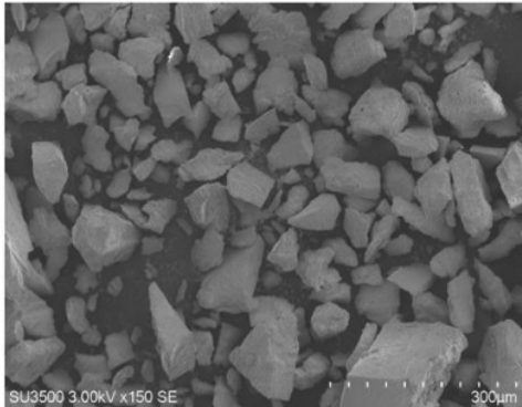
Figure 4 (a). Struvite formation using RATB
