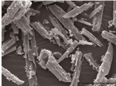
Figure 4 (b). Struvite formation using bulhead reactor
