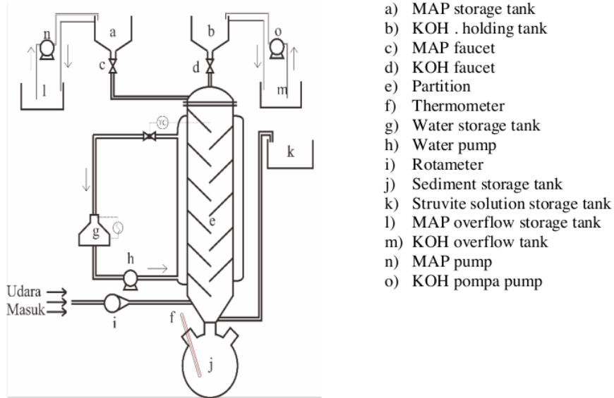
Figure 3. Bulk reactor arrangement
