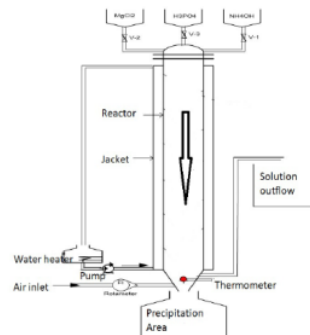
Figure 1. Schematic Diagram of Vertical Reactor
