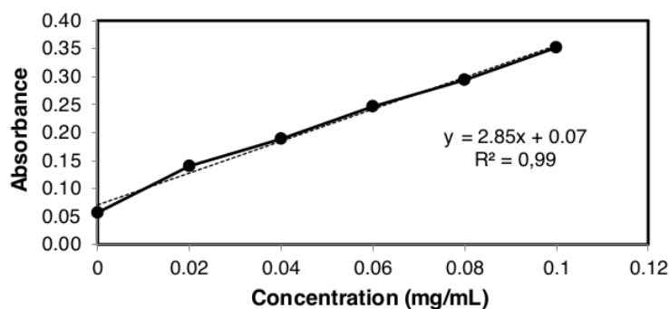
Figure 1. Standard curve of ascorbic acid
