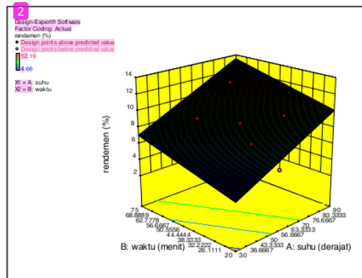
Gambar 2. 3D Surface Rendemen Pektin Pedada
