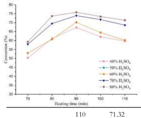
Fig. 1. Correlation between heating time and H 2 SO 4 concentration with Al 2 (SO 4 ) 3 conversion
