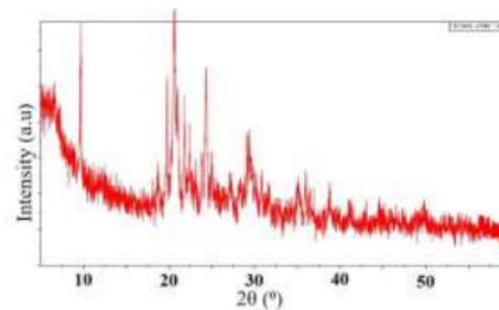
Fig. 2. The diffractogram of product obtained by Lapindo mud extraction
