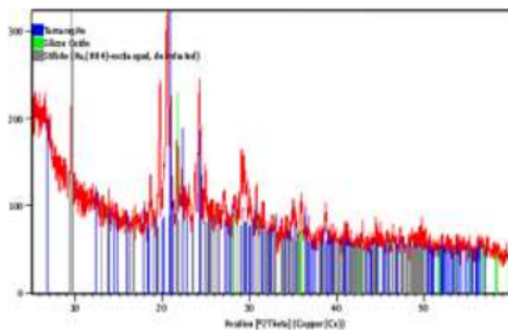
Fig. 3. Analysis using X-ray Diffraction (X-RD)
