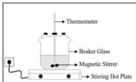
Fig. 1. The equipment of hydrolysis
