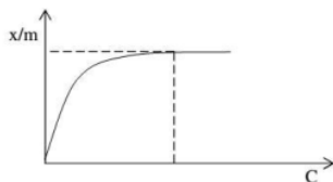
Figure 1. Langmuir adsorption isotherm curve (Handayani & Sulistyanto, 2009)
