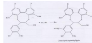
Gambar.2. Reaksi lignin + formaldehid (HCOH) → ortho-hydroxymethyl lignin
