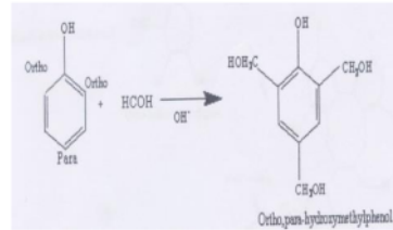
Gambar.1.Phenol+formaldehid→ortho,para hydroxymethylphenol
