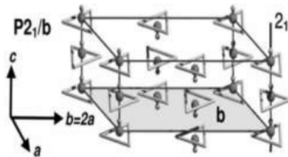
Fig. 1 Monoclinic Hydroxyapatite (HAp) Structure
