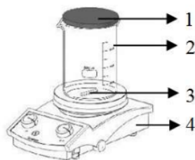
Fig. 3 The Set Up of Hydroxyapatite Synthesis
