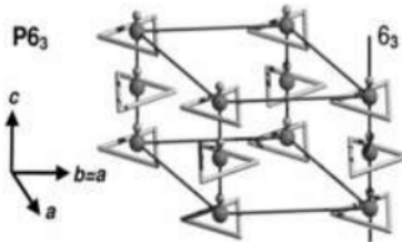
Fig. 2 Hexagonal Hydroxyapatite (HAp) Structure
