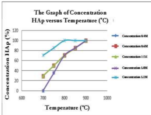
Fig. 4. The Graph of Concentration HAp versus Temperature (°C)
