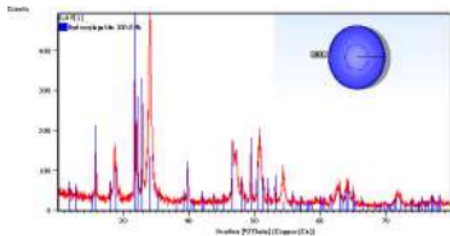
Fig. 5 The Graph of result Analisa XRD with Poshpate Acid Concentration 0.4M and Temperature 900 °C
