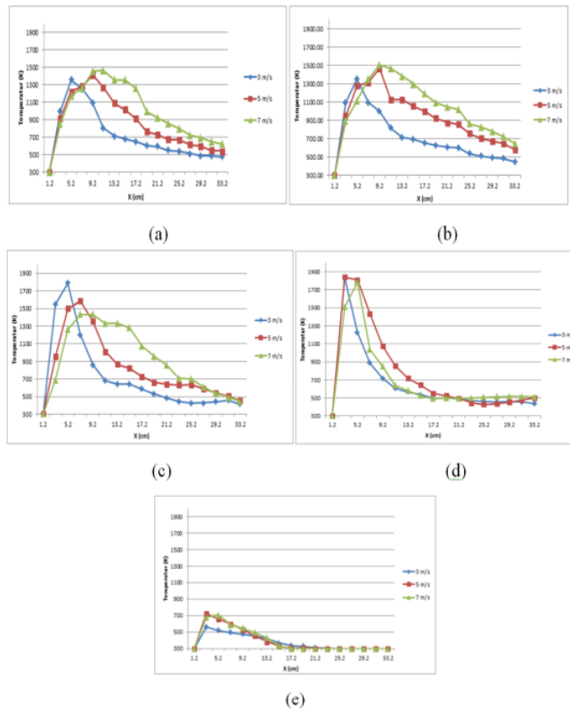
Figure 5. Temperature distribution graphic at different swirl vane configuration (a) without swirl vanes (b) 10^\circ (c) 30^\circ (d) 45^\circ and (e) 60^\circ as a function of flame height at different fuel velocity 3 , 5, and 7 m/s
