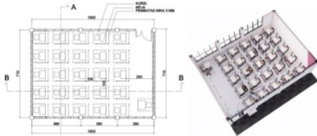
Gambar 7. Denah Ruang studio 3-1 tipe Rectangle
