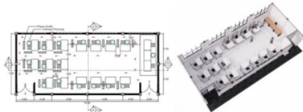
Gambar 15. Denah Ruang 4-1 tipe Horse Shoe
