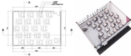
Gambar 8. Denah Ruang studio 3-1 tipe Semi Circle
