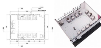
Gambar 10. Denah Ruang 3-1 tipe Horse Shoe
