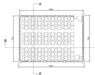
Gambar 5. Denah studio gambar 3-1 FAD
