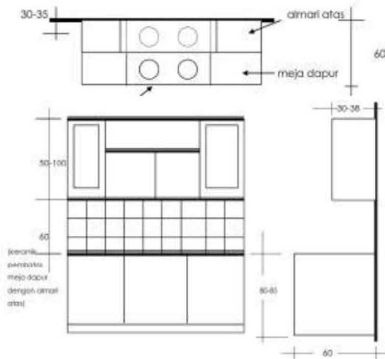
Gambar 12.27.detail almari dapur
