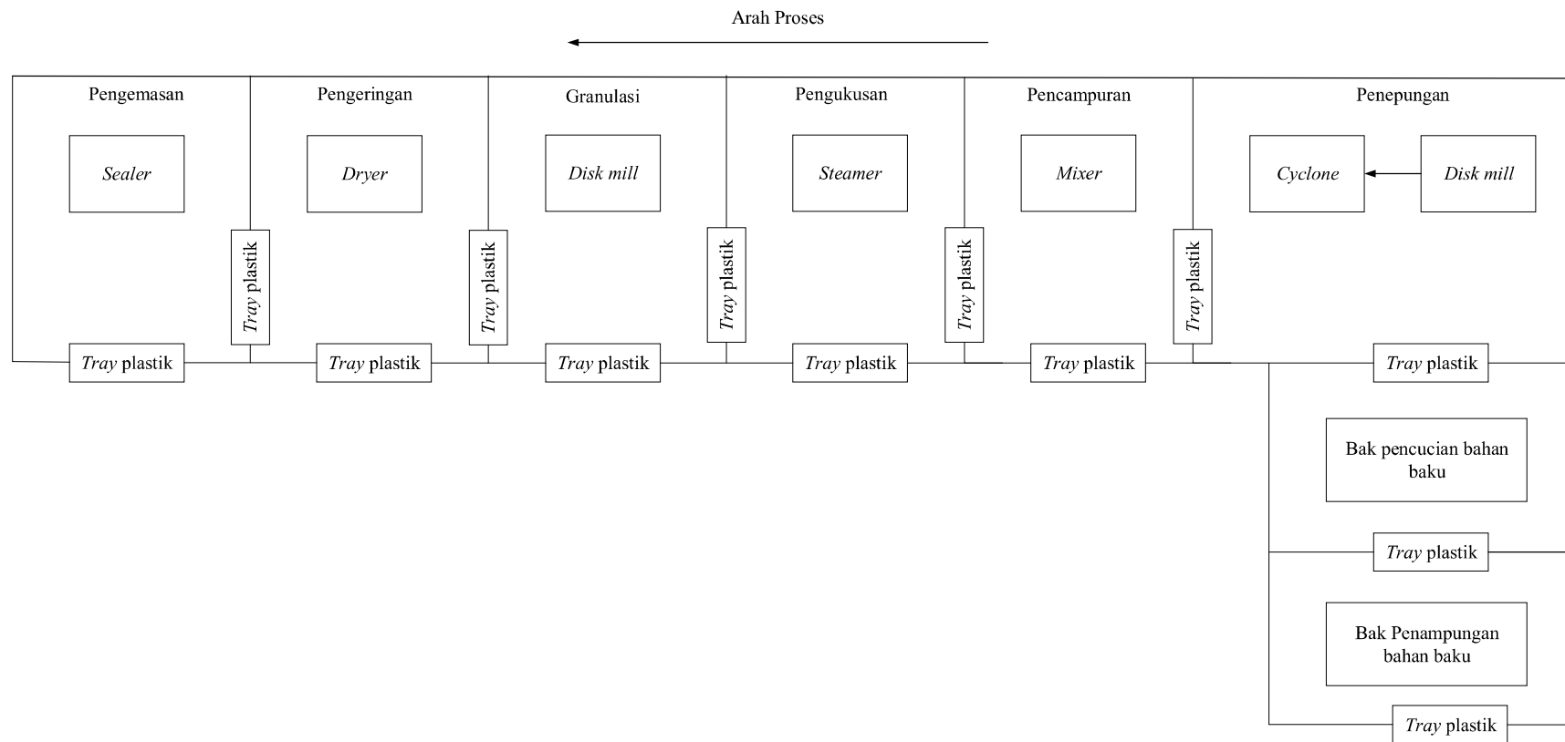
Gambar 4. Lay out peralatan CV. Riang Java Food
