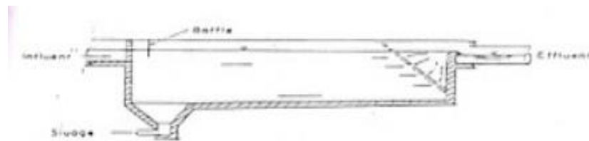
Gambar 2. 5 Bak Sedimentasi Rectangular
