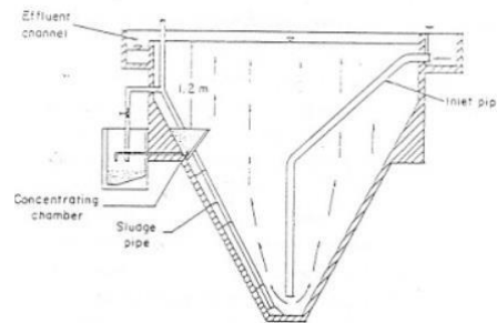
Gambar 2. 4 Bak Sedimentasi Circular Center Feed
