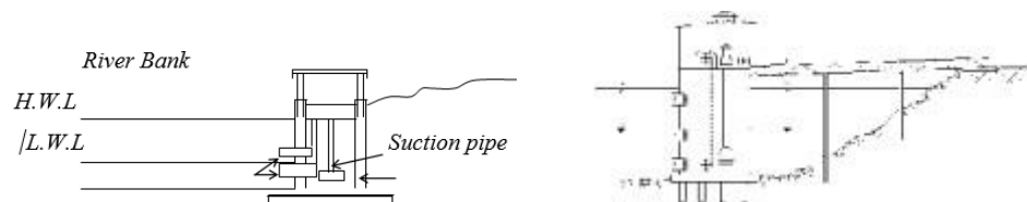
Gambar 2. 1 Shore Intake dan River Intake
