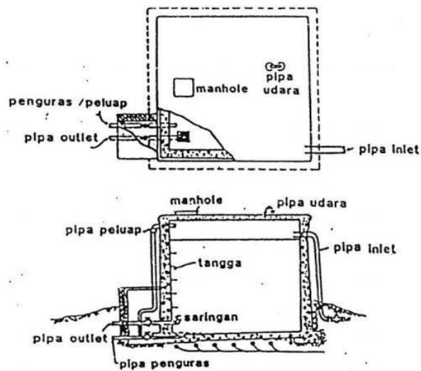
Gambar 2. 10 Reservoir Permukaan
