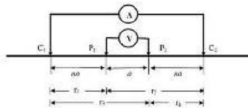
Fig. 2. Wenner-Schlumberger configuration
