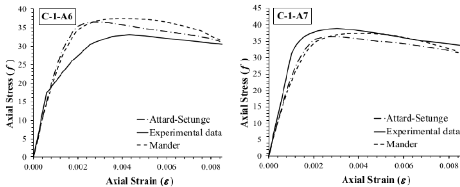
Fig. 4. Axial stress-strain curve for specimen ID C-1-A6 and C-1-A7
