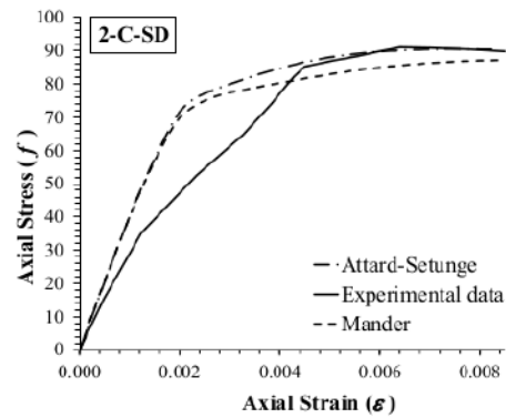
Fig. 8. Axial stress-strain curve for specimen ID 2-C-SD
