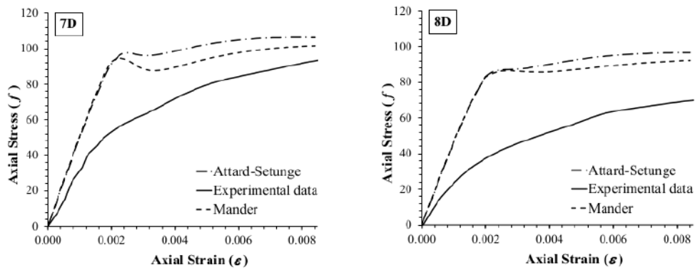
Fig. 3. Axial stress-strain curve for specimen ID 7D and 8D
