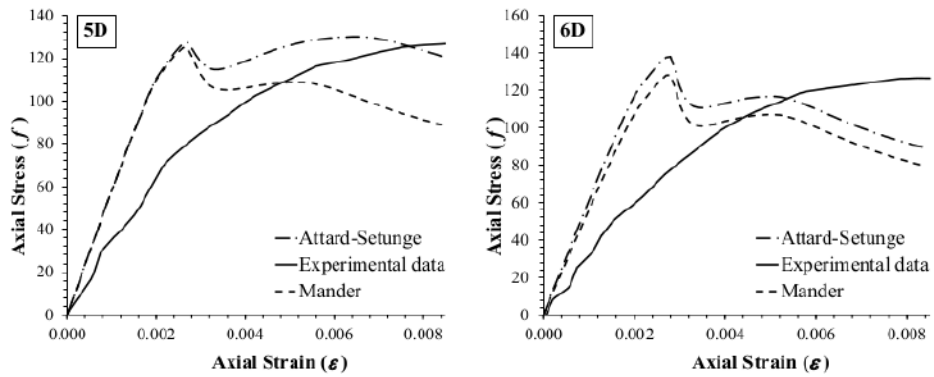
Fig. 2. Axial stress-strain curve for specimen ID 5D and 6D
