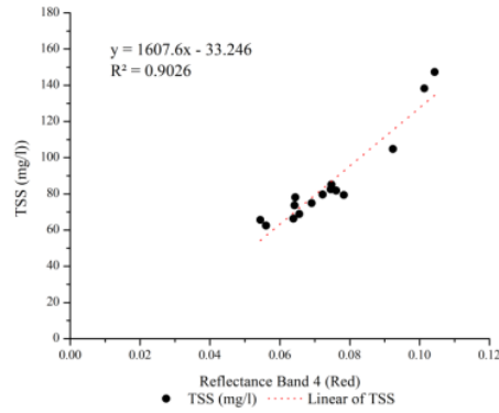
Figure 3. TSS distribution with Linear models at Band 4 (red)
