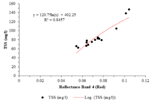
Figure 5. TSS distribution with Logarithmic models at Band 4 (red)
