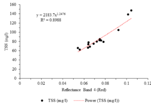
Figure 6. TSS distribution with Power models at Band 4 (red)
