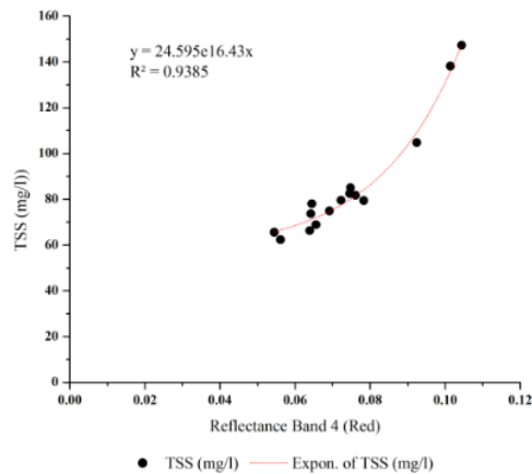
Figure 4. TSS distribution with Exponent models at Band 4 (red)
