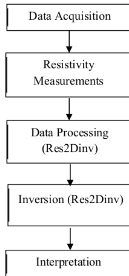
Fig.5. Research methodology
